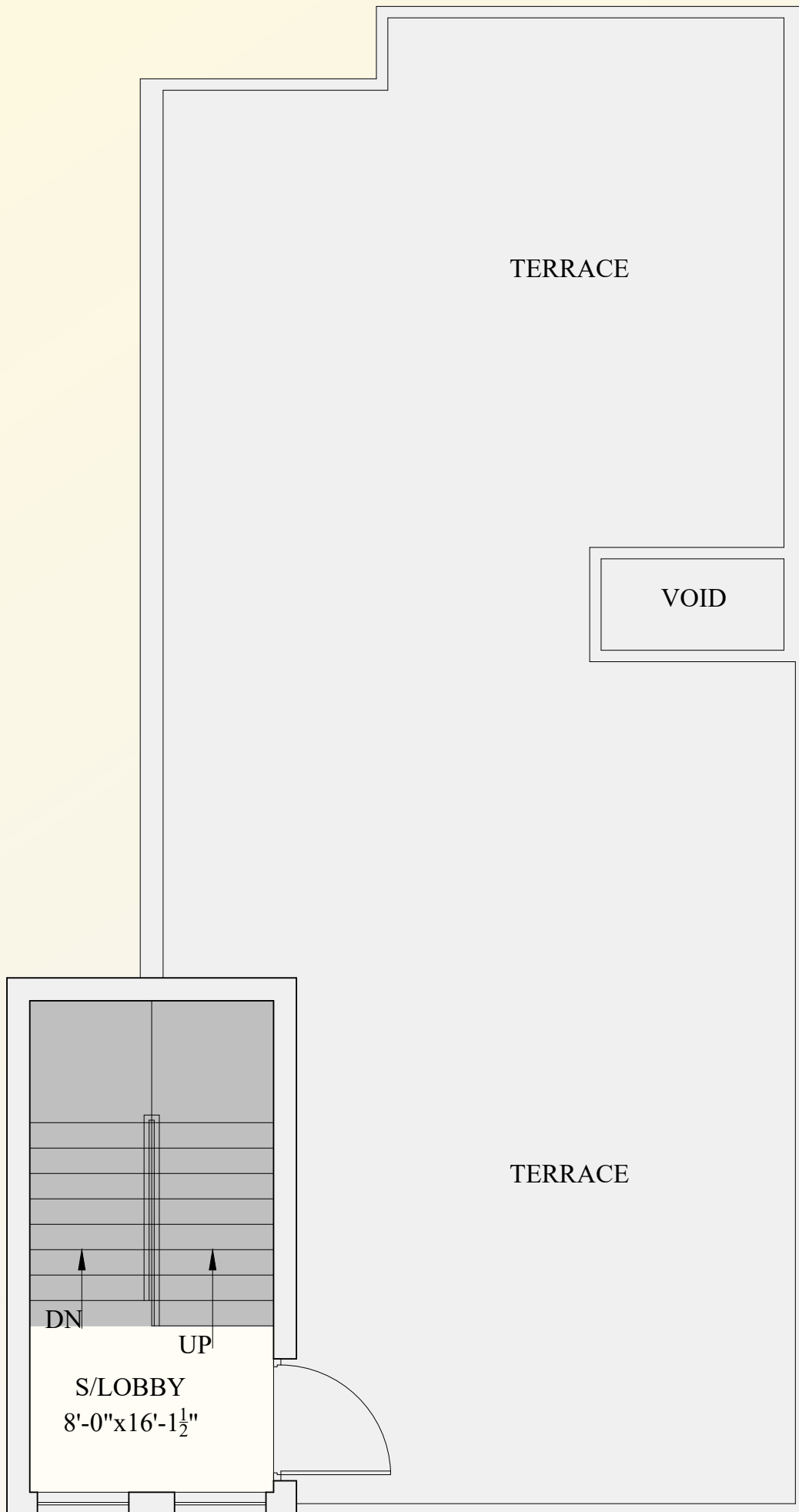
ROOF PLAN
